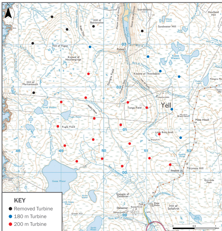
REVISED WIND FARM LAYOUT
