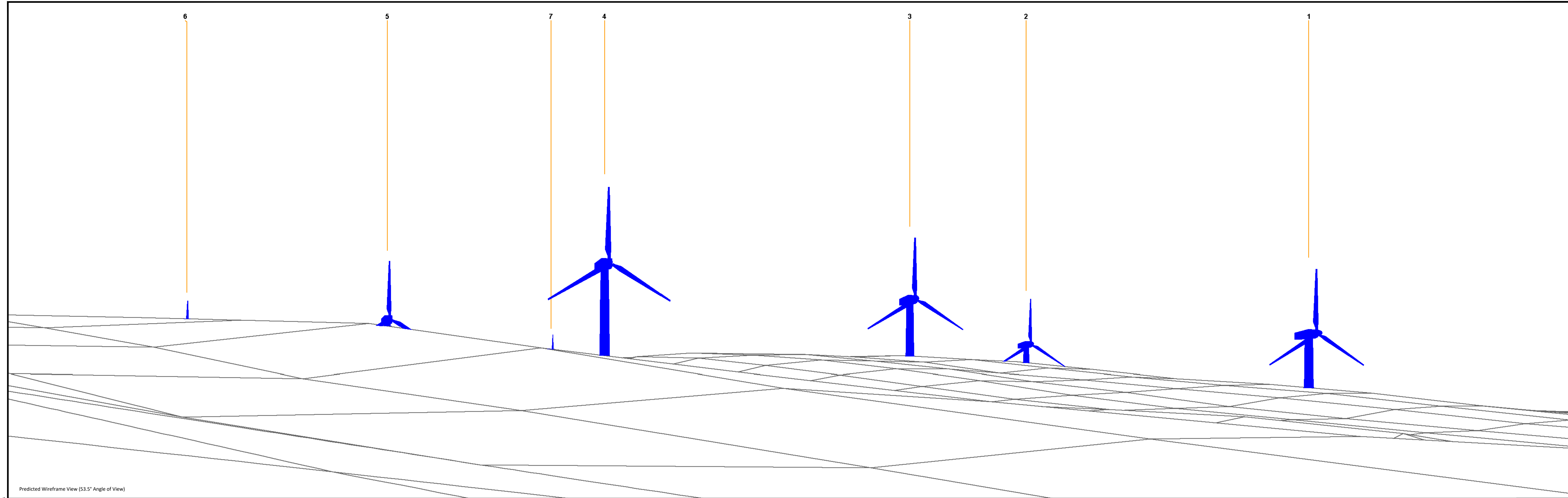
Figure 5.8.5d(ii) - RVAA Settlement Cluster 5: East Gloop, scattered properties on the minor road east of Gloop View flat at a comfortable arms length. The principal distance is 812.5mm
