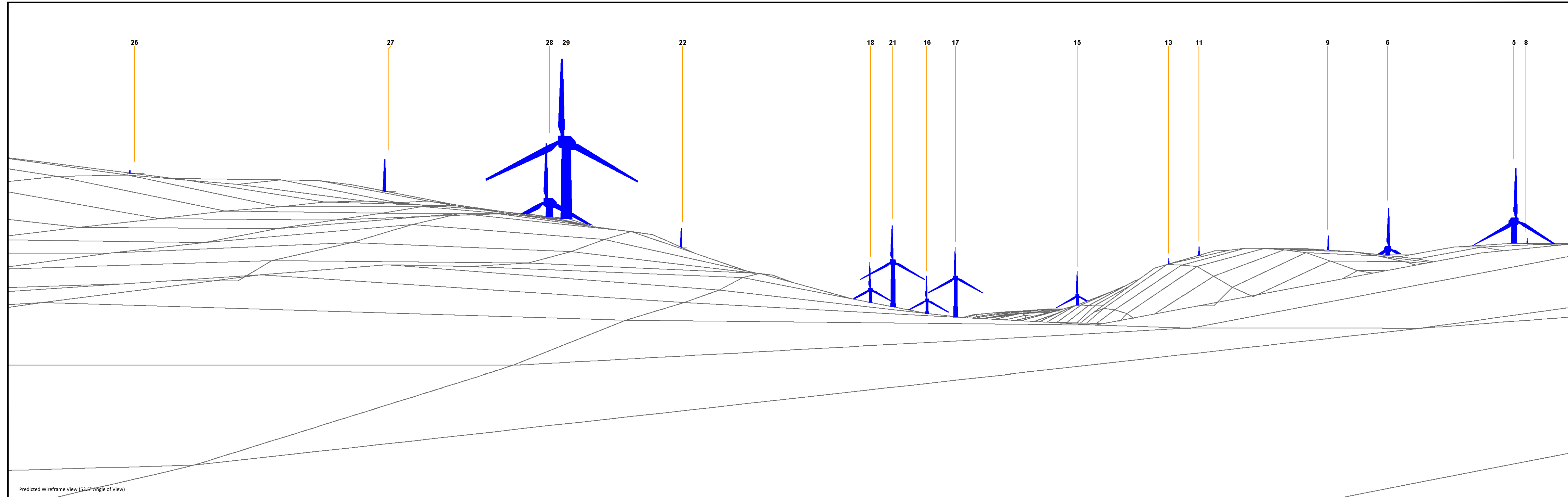
Figure 5.8.4d(i) - RVAA Settlement Cluster 4: North Gloup, including Kirks (The Kirks) View flat at a comfortable arms length. The principal distance is 812.5mm
